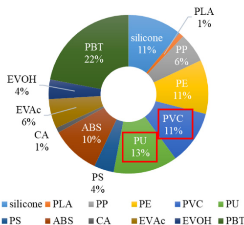
Figure 3. Relative abundance of polymer types identified in moss samples from the MADAME project (Hayes et al. 2024 - preliminary findings from the MADAME project).
